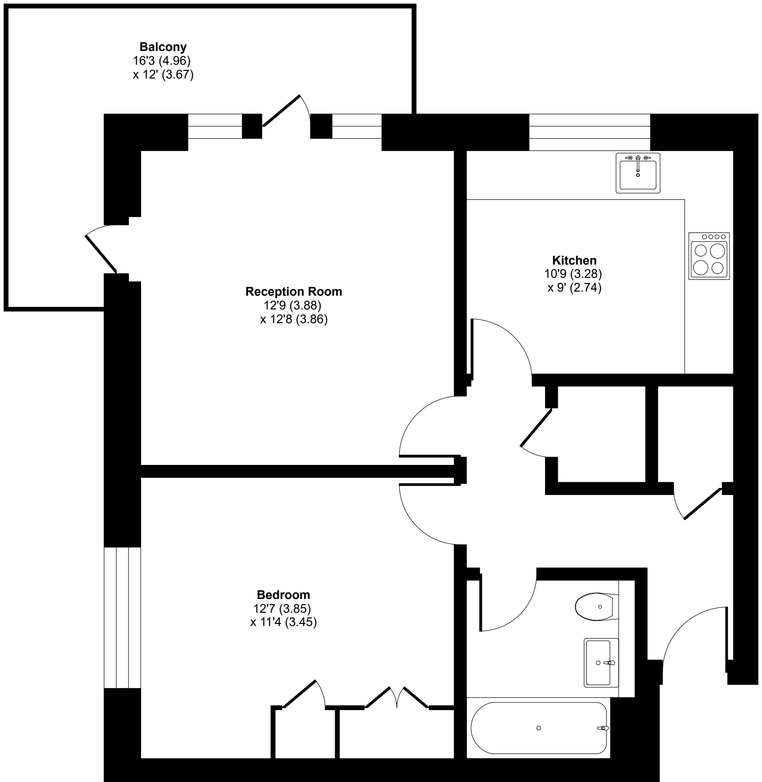
SECOND FLOOR
